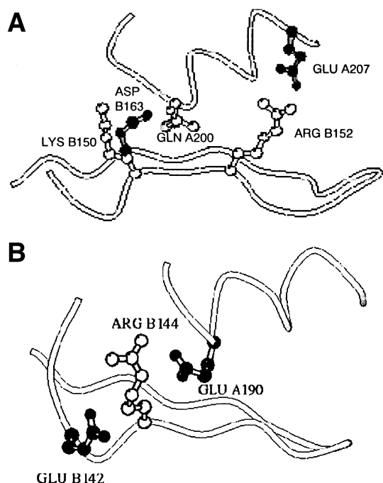
Fig. 2. A: Model of the E. coli IPMDH showing the side chain of Gln-200 and some charged residues in its proximity. The ribbon represents the protein backbone. When Gln-200, located at the N-terminus of a helical region, is mutated to Glu (in subunit A), it can form an intersubunit ion pair with either Lys-B150 or Arg-B152, both located in the arm-like region of subunit B. Both these residues themselves form ion pairs with other charged side chains: Lys-B150 forms an ion pair with Asp-B163 in the same subunit (subunit B); and Arg-B152 forms an ion pair with Glu-A207 in the other subunit (subunit A). Glu-A207 is part of a larger ion cluster (not shown). Because of the symmetry of the dimer, the same situation is observed when Gln-200 is mutated to Glu in subunit B. B: Model of the T. thermophilus IPMDH showing the side chain of Glu-190 and some charged residues in its proximity. The ribbon represents the protein backbone. When Glu-190 is mutated to Gln (in subunit A), the intersubunit ion pair with Arg-B144 and thus the three-member ion cluster (formed also by Glu-B142) is disrupted.
