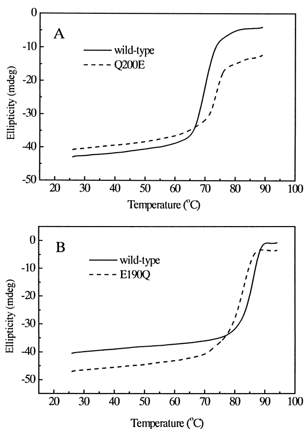
Fig. 4. Unfolding of (A) the E. coli (solid line, T_{tr}' = 69.7^\circ\text{C} ) and of its Q200E mutant (dashed line, T_{tr}' = 73.7^\circ\text{C} ) IPMDHs and (B) of the T. thermophilus (solid line, T_{tr}' = 86.2^\circ\text{C} ) and of its E190Q mutant (dashed line, T_{tr}' = 83.0^\circ\text{C} ) IPMDHs followed by CD spectroscopy at 221 nm. The raw data were smoothed. The transition temperatures obtained this way show the increased stability of the mutant IPMDH. The measurement was carried out in pH 7.6 potassium phosphate buffer containing 0.3 M KCl, at a protein concentration of 0.4 mg/ml. The heating rate was 50^\circ\text{C/h} .
