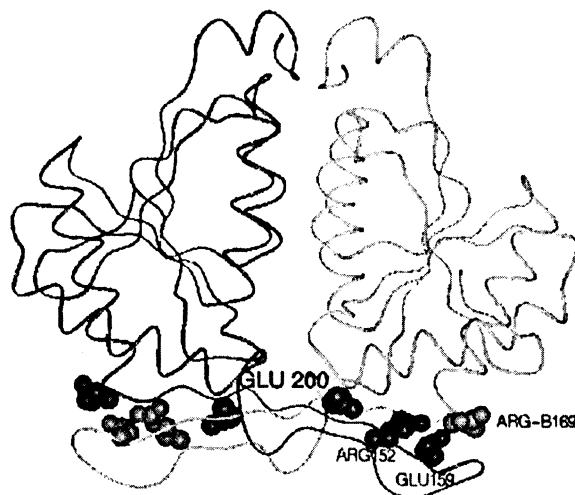
Fig. 1. Ribbon diagram of mesophilic ( E. coli ) IPMDH. The residues visualized by the spacefilling model constitute the ion cluster formed at the subunit interface, upon replacement of Gln-200 by Glu.
