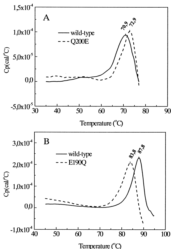
Fig. 3. Partial heat capacity curves of (A) the E. coli (solid line, T_m' = 70.9^\circ\text{C} ) and of its Q200E mutant (dashed line, T_m' = 72.9^\circ\text{C} ) IPMDHs and (B) the T. thermophilus (solid line, T_m' = 87.8^\circ\text{C} ) and of its E190Q mutant (dashed line, T_m' = 83.8^\circ\text{C} ) IPMDHs. The measurements were carried out with a heating rate of 50^\circ\text{C/h} in pH 7.6 potassium phosphate buffer containing 0.3 M KCl, the protein concentration was 0.4 mg/ml. The unfolding was irreversible.
